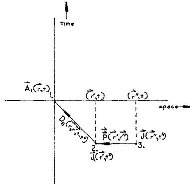
FIG. 2. \mathbf{A}_\perp(\mathbf{r}, t) , the vector potential in the Coulomb gauge, is built up from contributions of the transverse current density \mathbf{J}_\perp(\mathbf{r}', t') which propagate with the speed of light from the points (\mathbf{r}', t') . \mathbf{J}_\perp(\mathbf{r}', t') is the formal result of an instantaneous propagation of \mathbf{J}(\mathbf{r}'', t'') from the points (\mathbf{r}'', t'') to (\mathbf{r}', t') .
