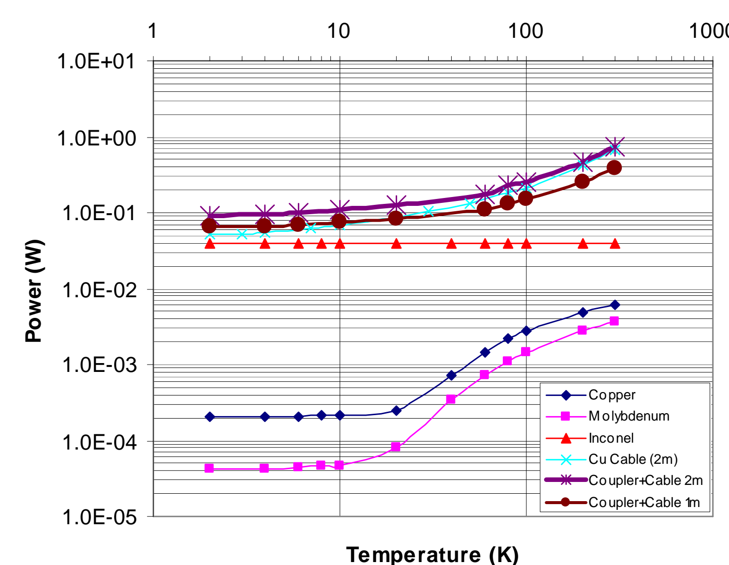
Figure 3: Power losses (4W RF) in coupler antenna (Cu, Mo, & In) and coaxial cable (medium dia) as a function of temperature. Also shown is the total power loss for 1m and 2m cable lengths.
