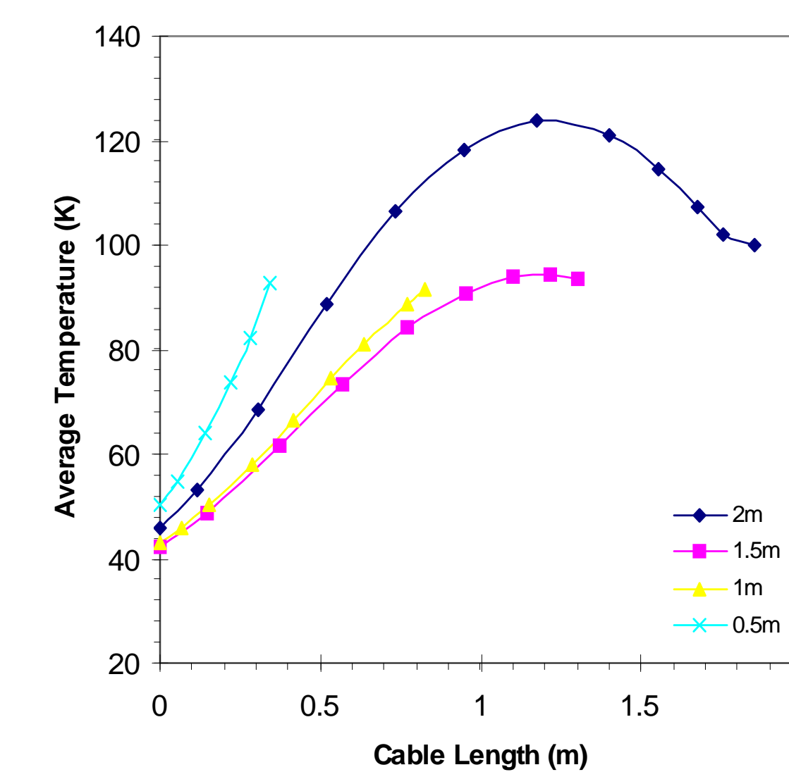
Figure 11: Dynamic temperature distribution in cable for different cable lengths up to 80K point (10W RF, large dia. cable).
