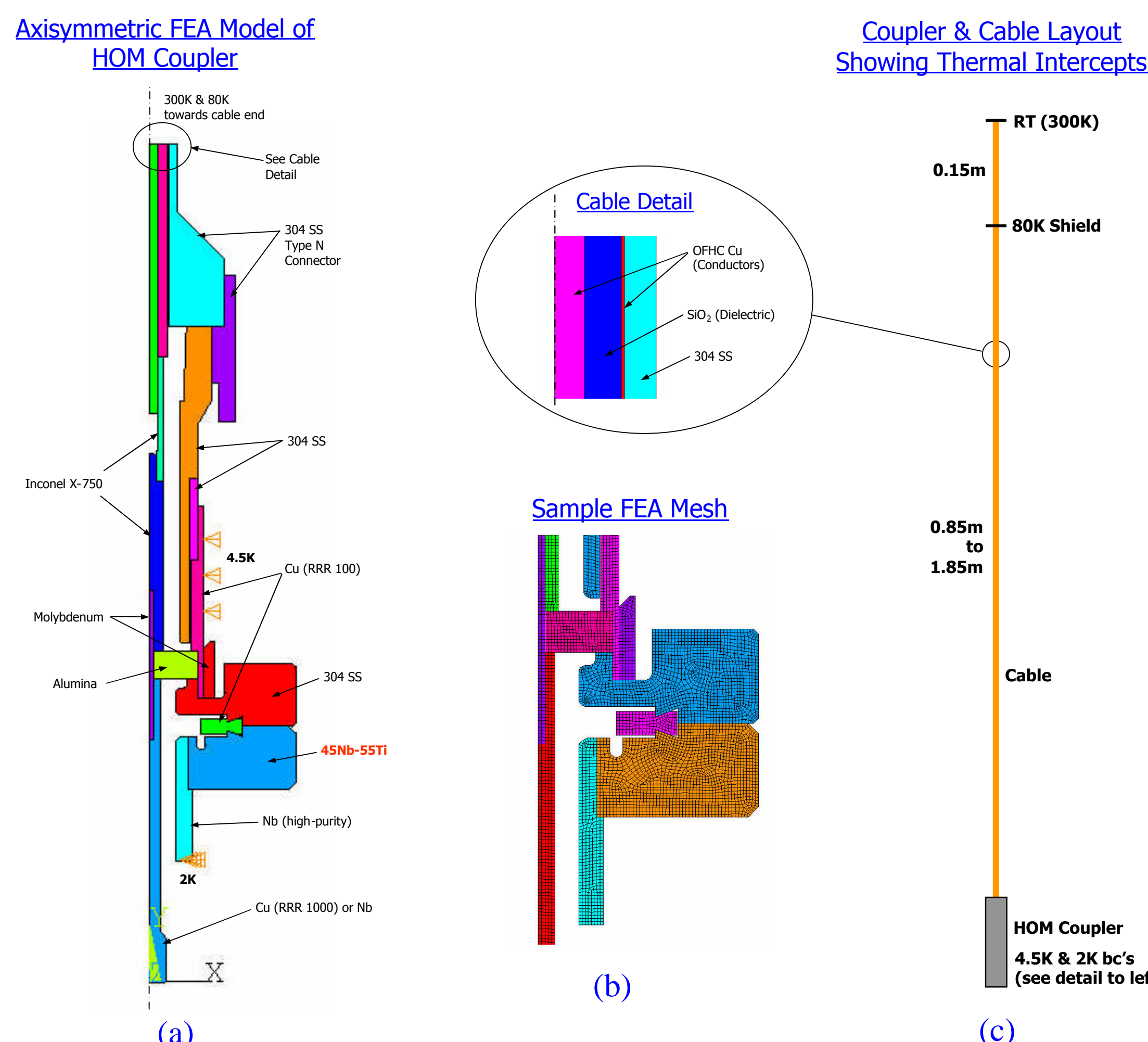
Figure 1: Axisymmetric FEA Model of FNAL HOM Coupler, showing cable section details, FEA mesh, and thermal intercepts.
