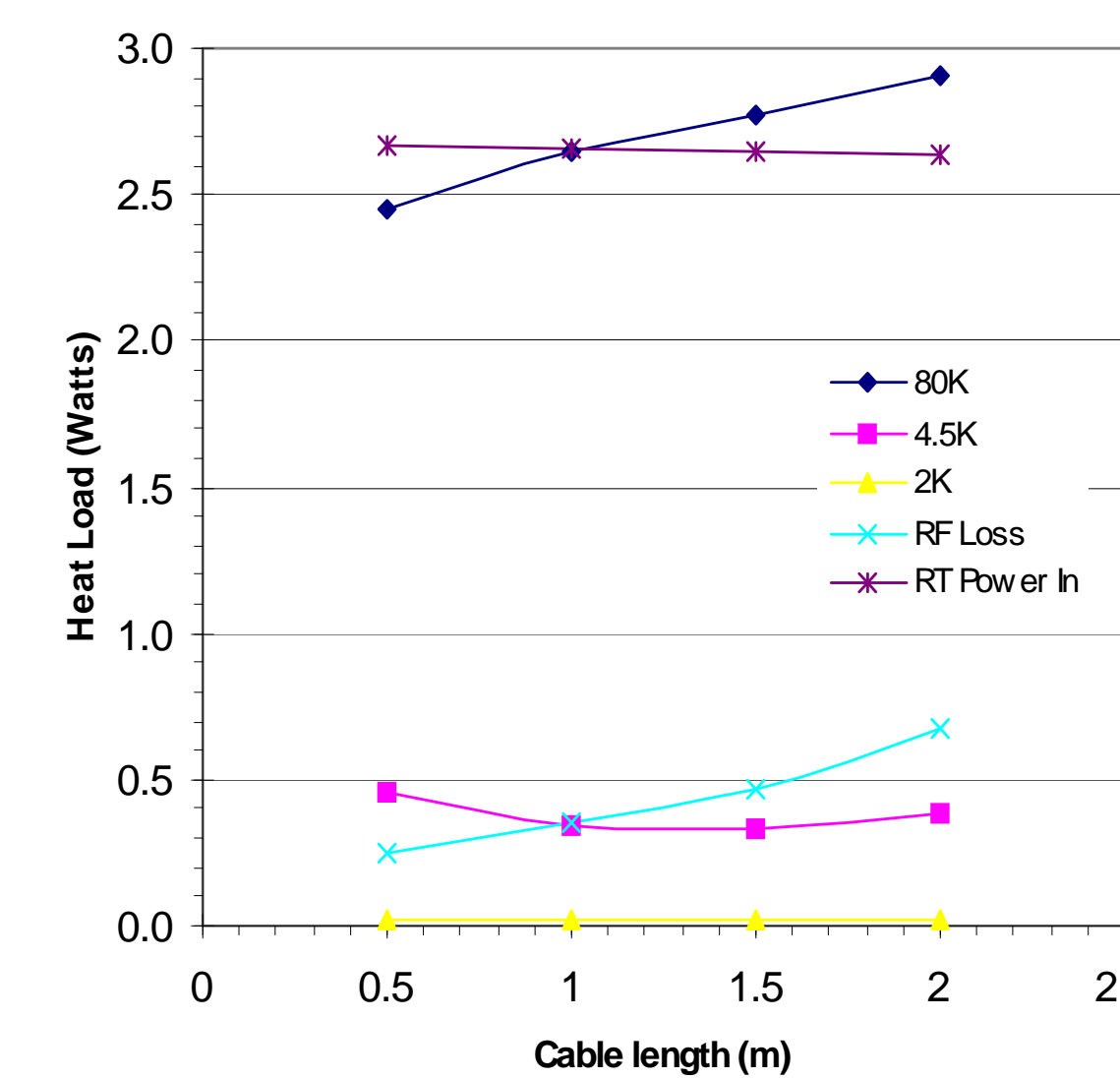
Figure 10: Dynamic heat loads as a function of cable length at the different junctions (10W RF, large dia. cable).
