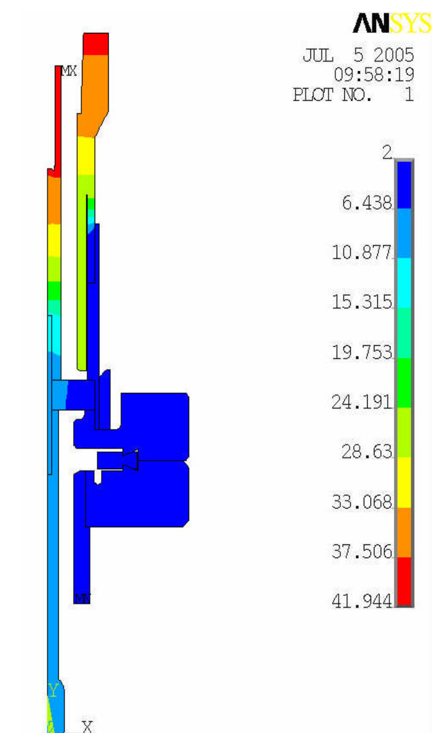
Figure 13: Dynamic temperature contour plots in coupler for 1.5m cable length (10W RF, medium dia. cable).
