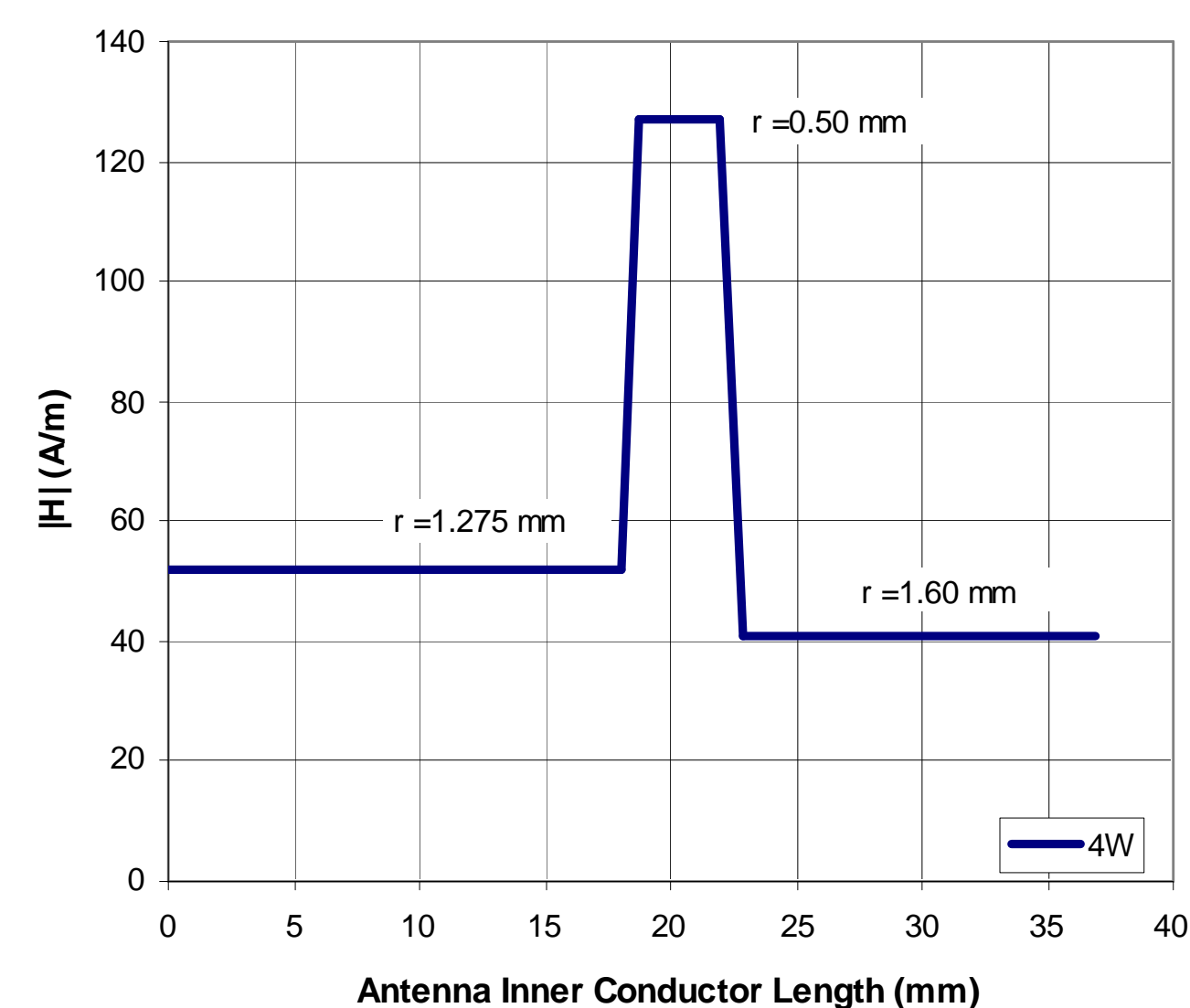
Figure 2: Magnetic field intensity in the antenna (inner conductor) at 4W power.
