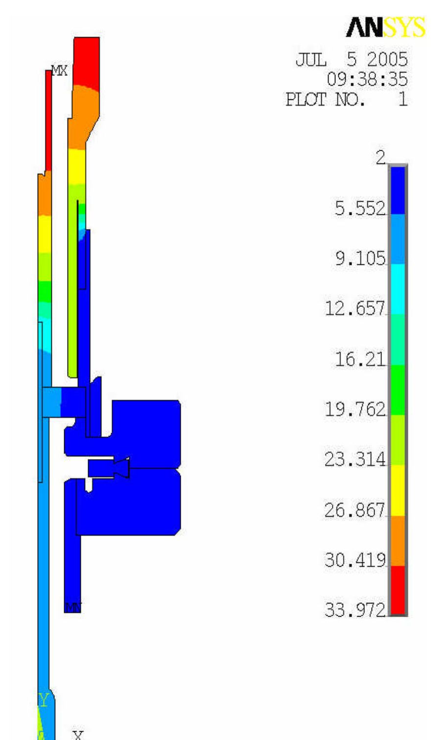
Figure 12: Dynamic temperature contour plots in coupler for 1.5m cable length (4W RF, small dia. cable).
