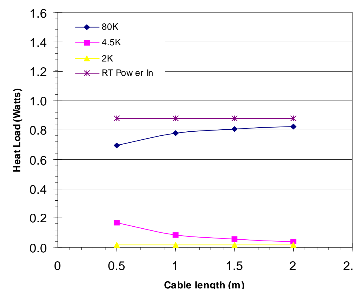
Figure 8: Static heat loads as a function of cable length at the different junctions (small dia. cable).
