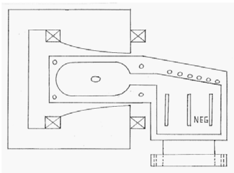
Figure 1 Possible magnet and vacuum chamber for the HER and LER of a SBF.
