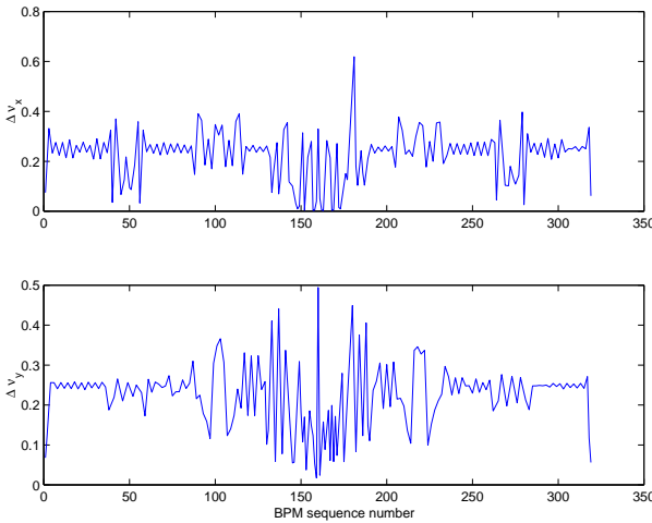
Figure 10: The phase advances with a reduced skew (SK4) value that shows reduced beta beatings. Note that at the arcs, the ideal phase advances should have the same values. (BPM buffer data acquired on April 9, 2002 from the PEP-II LER.)
