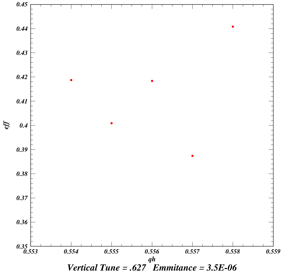
FIGURE 8. Efficiency using current qtunes and emittance, with pretzel amplitude reduced to zero. Horizontal qtune .556, vertical qtune .627, and emittance 3.5E-06 gives efficiency of 42%. Machine studies give efficiency of 38% for identical parameters.
