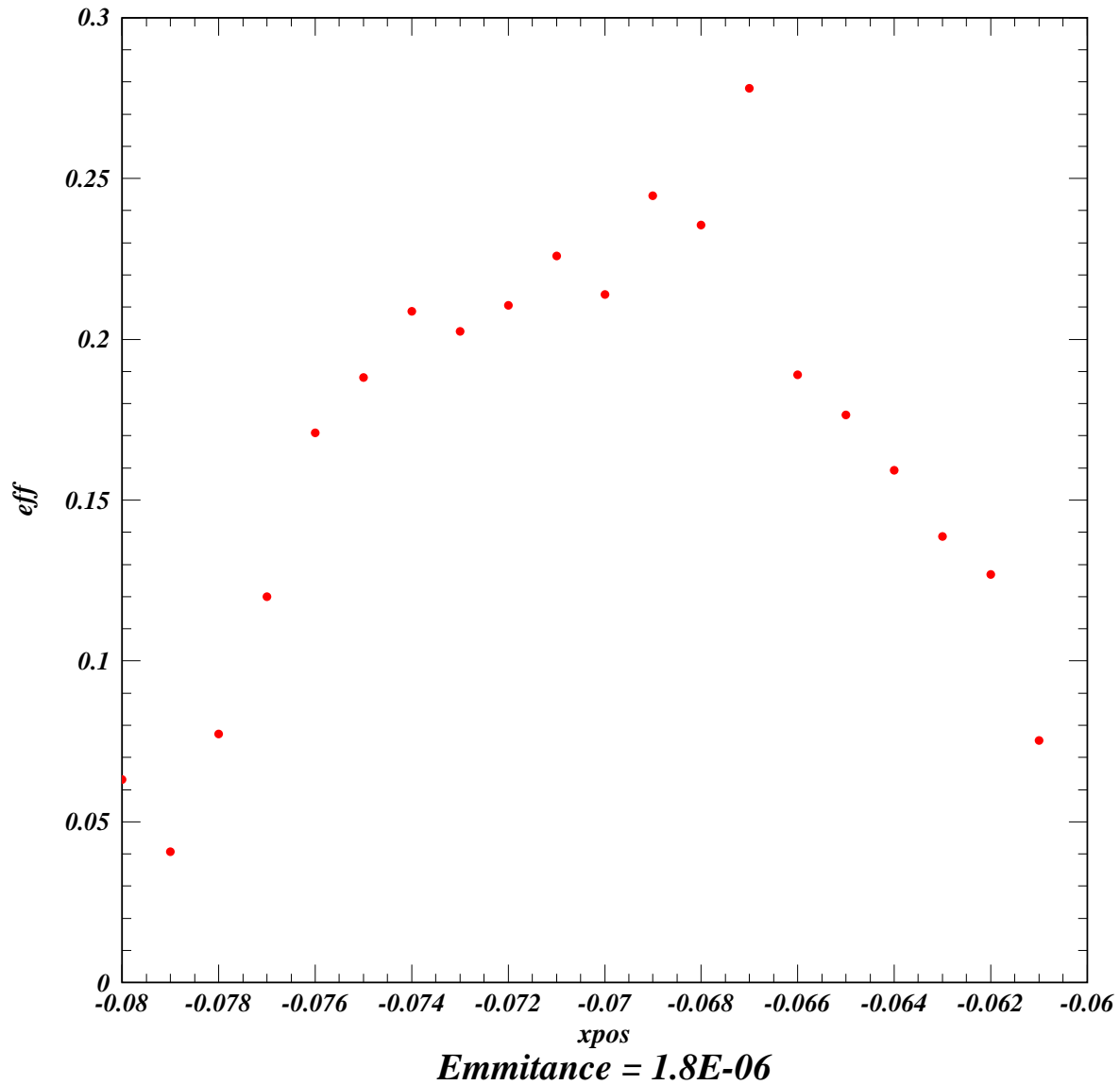
FIGURE 6. Efficiency variation with injection position, with improved emittance. INJTRACK suggested value of -0.071 m yields 23% efficiency. Ideal position of -0.067 m yields efficiency of 28%. Former lattice value of -0.055 yields efficiency of 0%.
