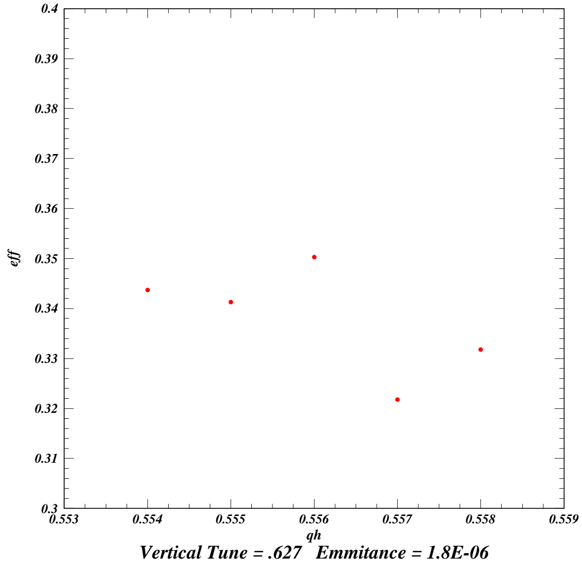
FIGURE 3. Calculation of efficiency after installation of beryllium vacuum windows, with present qtunes. 35% for horizontal qtune .556, vertical qtune .627, emittance 1.8E-06.
