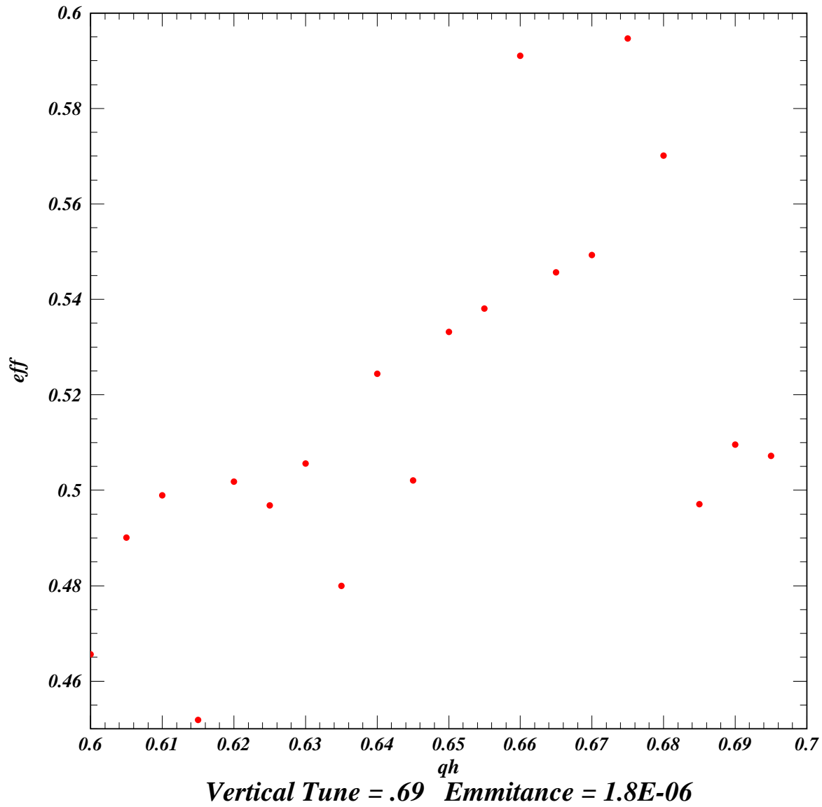
FIGURE 5. Efficiency for alternate qtunes and post installation emittance. 59% efficiency using horizontal qtune .675, vertical qtune .690, emittance 1.8E-06. 3,000 particles used to reduce statistical error.
