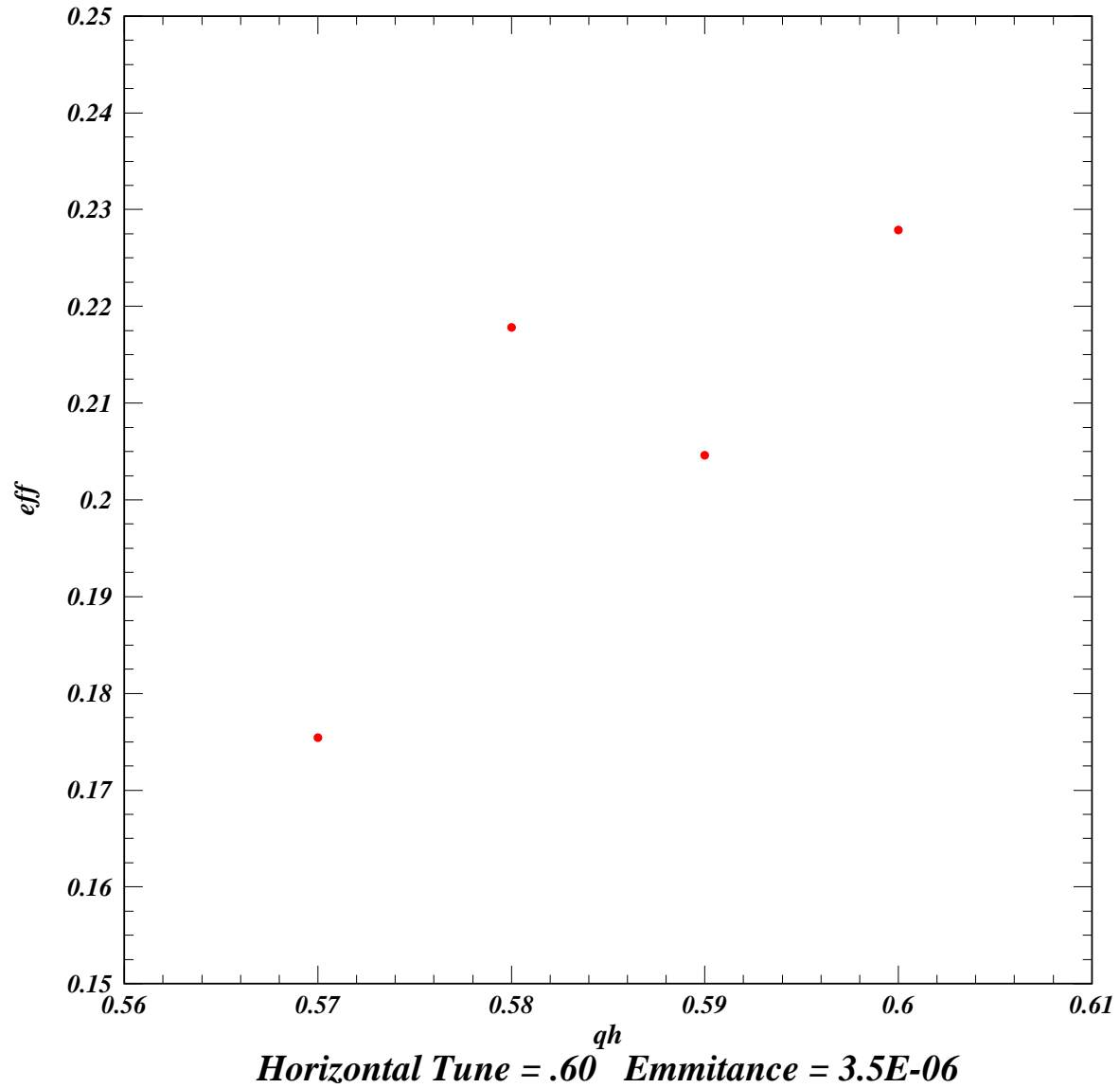
FIGURE 4. Efficiency for alternate qtunes and current emittance. 23% efficiency for horizontal qtune .600, vertical qtune .600, emittance 3.5E-06.
