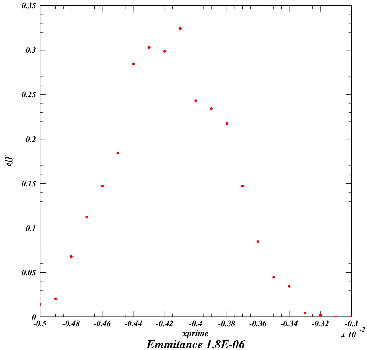
FIGURE 7. Efficiency variation with injection angle, with improved emittance. INJTRACK suggested value of -0.0044 rad yields efficiency of 28%. Ideal value for old lattice and current lattice of -0.0041 rad yields efficiency of 33%.
