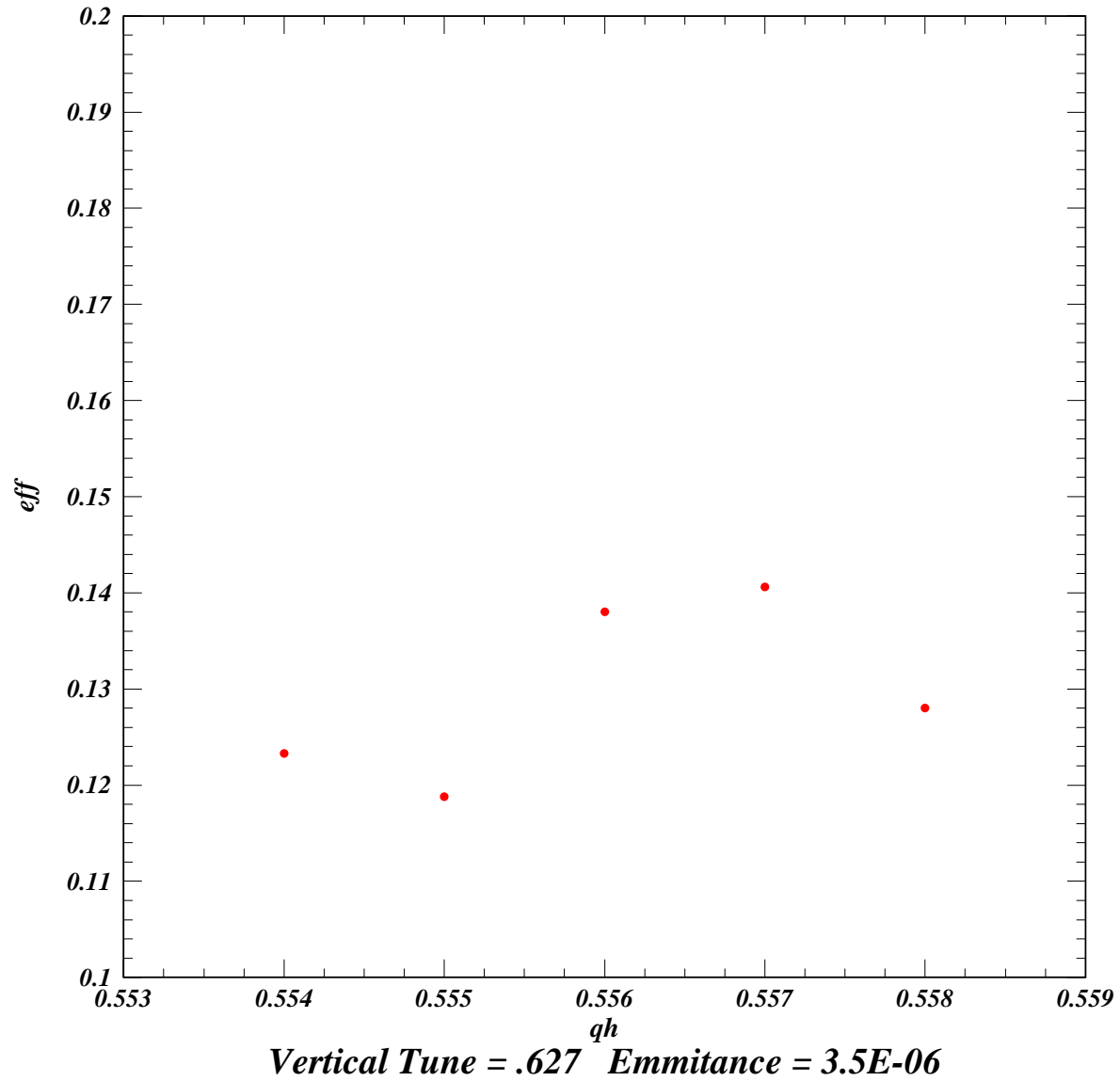
FIGURE 2. Calculation of efficiency using present qtunes and emittance value. 14% efficiency for horizontal qtune .556, vertical qtune .627, emittance 3.5E-06.
