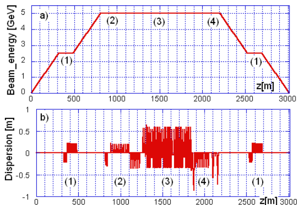
Figure 1: Beam energy (a) and horizontal dispersion (b) along the ERL.
