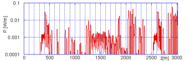
Figure 4: Total radiation power generated by the beam loss along ERL. \sim 99.8\% of the radiation generated by IBS particles
