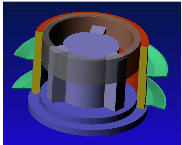
Figure 3: Pictorial representation of the use of the assembly fixture. (Ferrite ID is 3” with a nominal 0.030” wall.)
