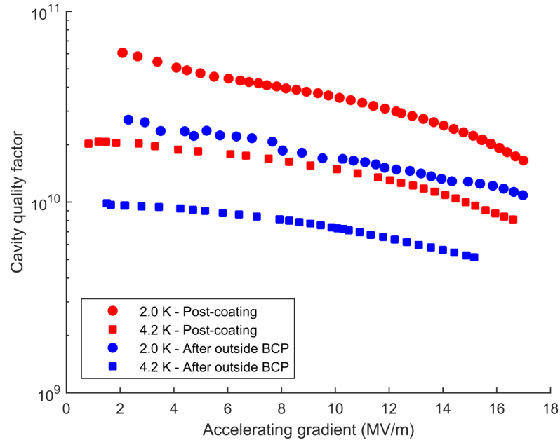
Figure 6.5: Q vs E of a \text{Nb}_3\text{Sn} cavity immediately post-coating and after a short outside BCP to remove the outside layer of \text{Nb}_3\text{Sn} .
