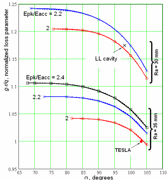
Figure 3: Normalized loss parameter for different angles of slope. Solid lines are for max G \cdot R/Q , dash lines are for minimal h . (Graphically both lines nearly overlap).
