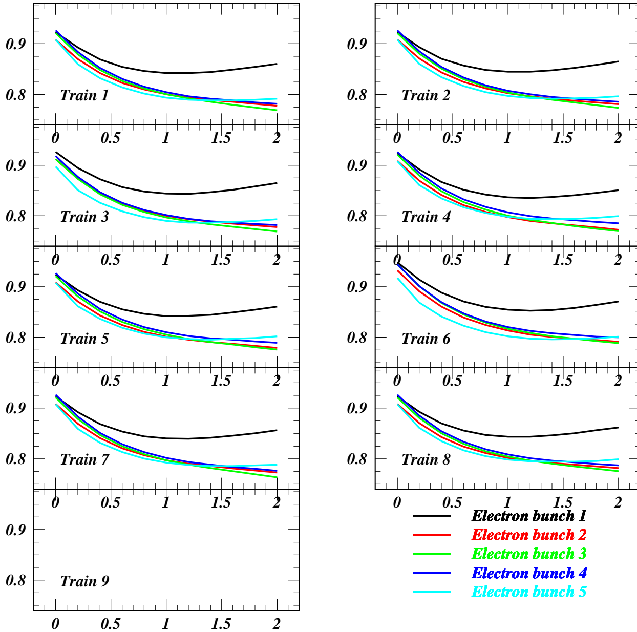
Vertical Beam Size from \beta at IP ( \mu ) vs e^+ Current (mA/bunch) for Job 1623
