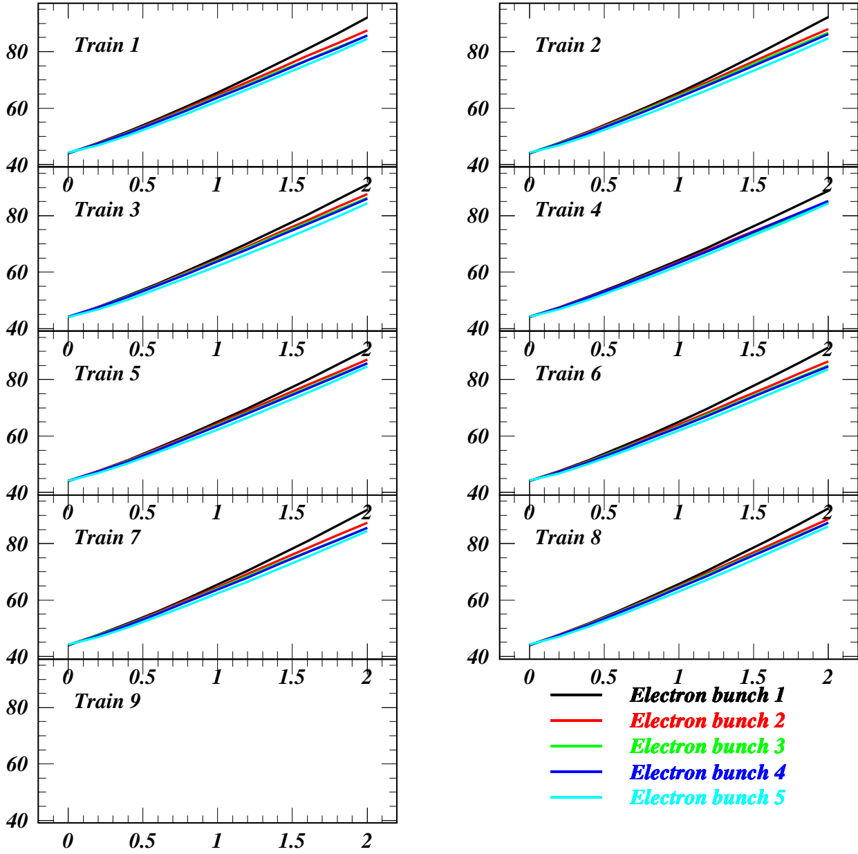
Vertical \beta_{max} (m) vs e^+ Current (mA/bunch) for Job 1623
