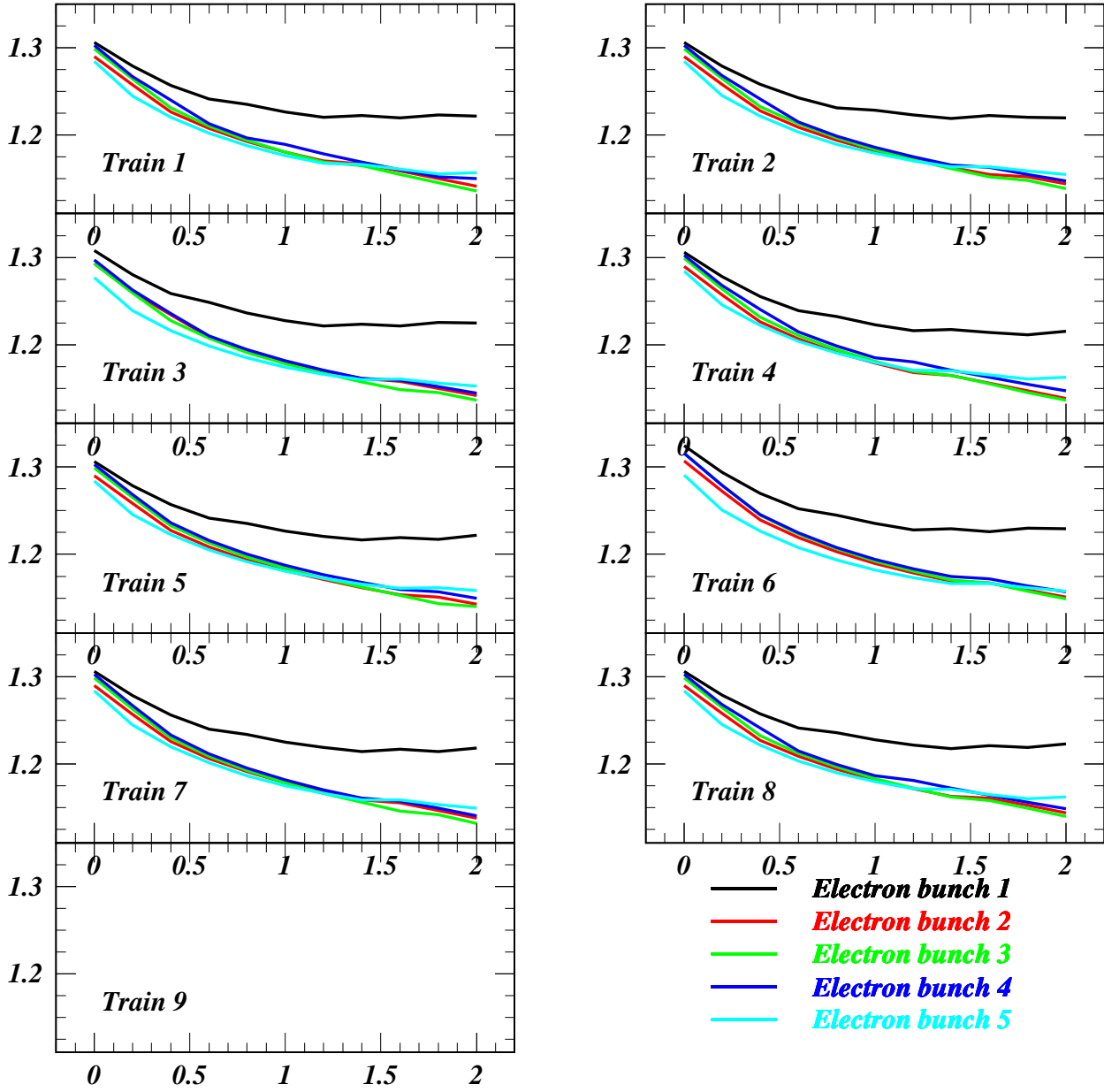
Vertical Beam Size at IP ( \mu ) vs e^+ Current (mA/bunch) for Job 1623
