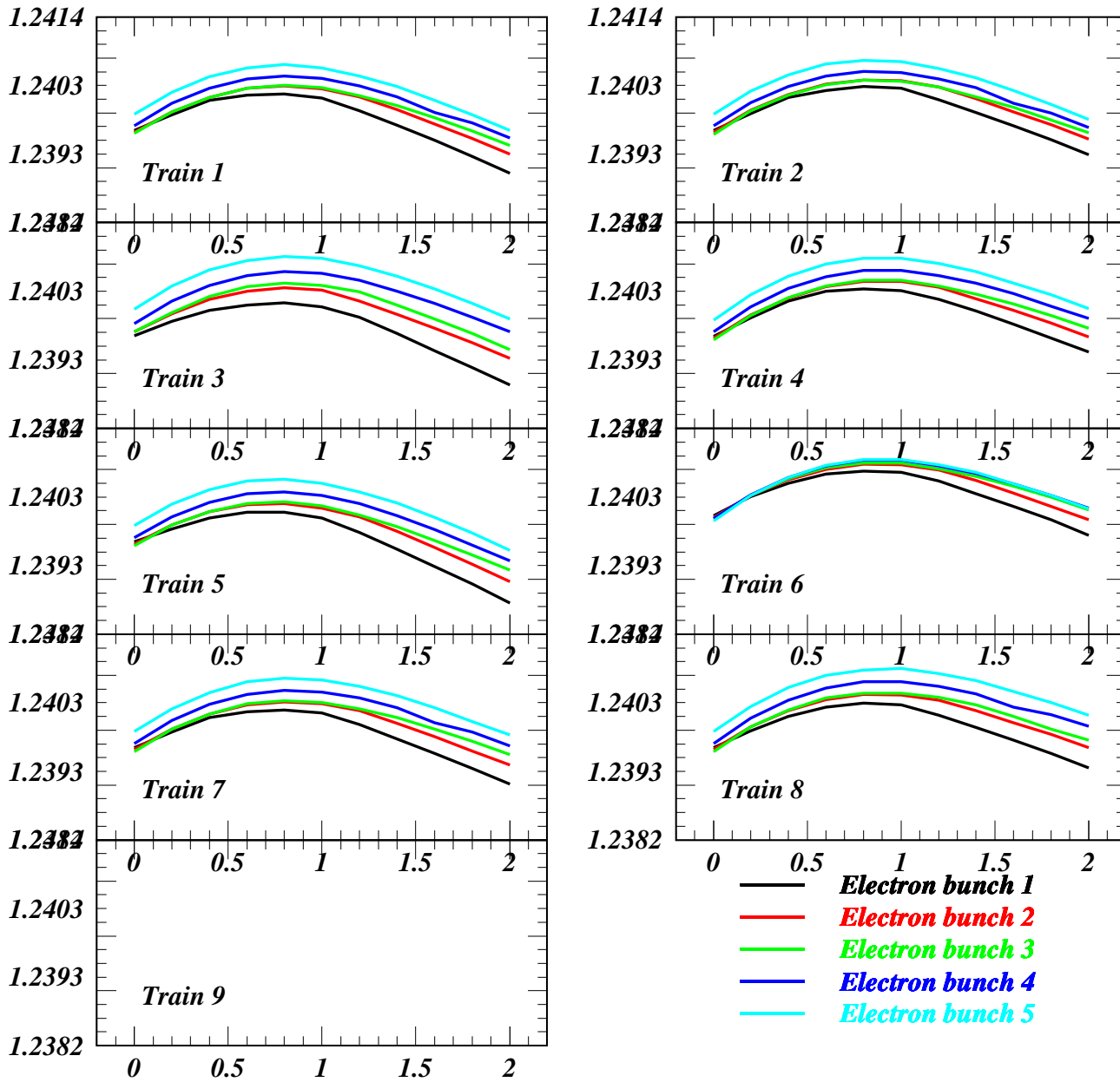
Bunch Length (cm) vs e^+ Current (mA/bunch) for Job 1623
