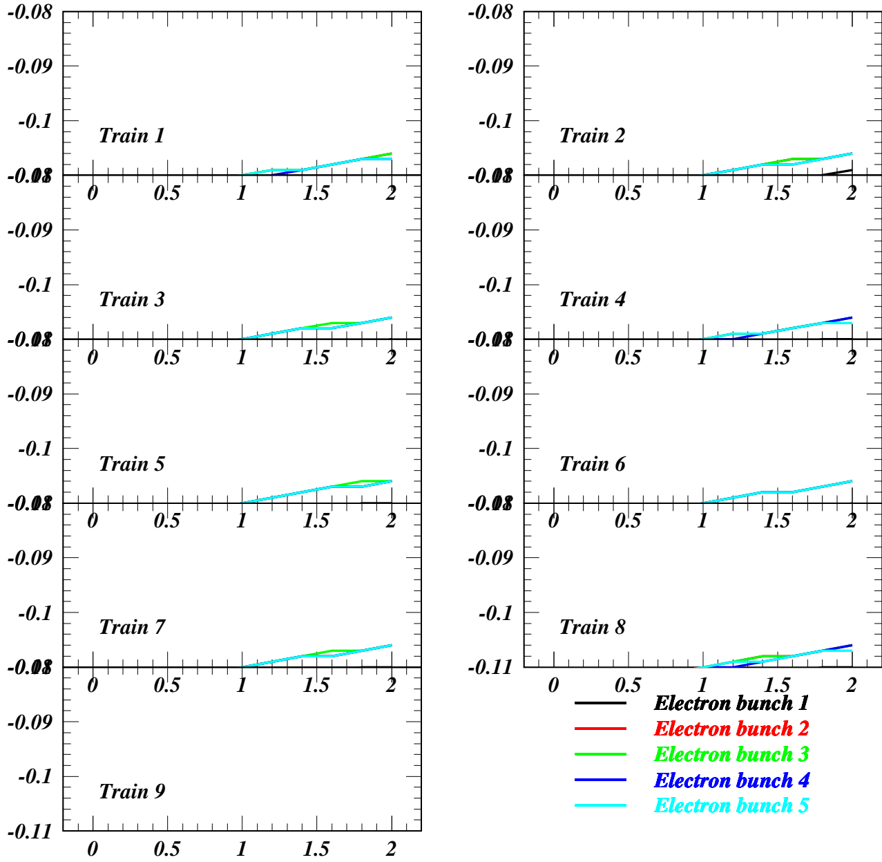
Vertical \eta^* (cm) vs e^+ Current (mA/bunch) for Job 1623
