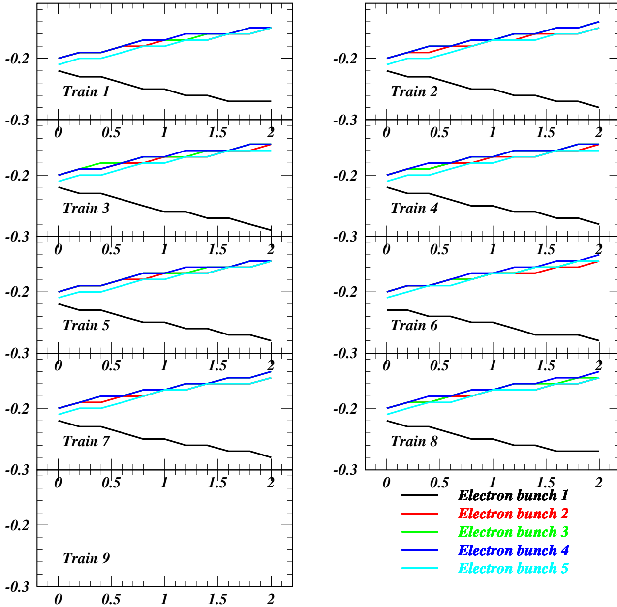
Vertical Crossing Angle (mrad) vs e^+ Current (mA/bunch) for Job 1623
