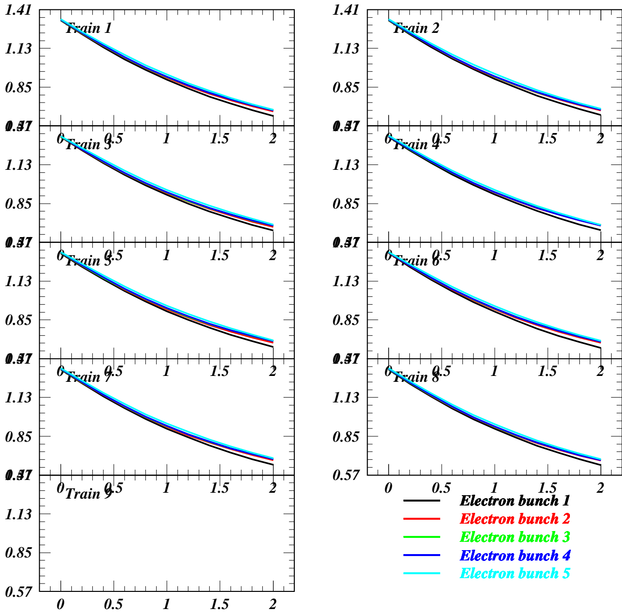
Vertical \beta^* (cm) vs e^+ Current (mA/bunch) for Job 1623
