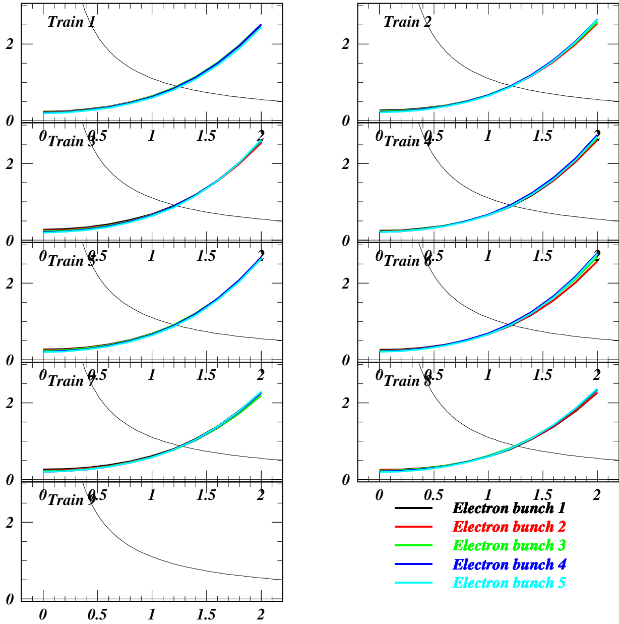
Welch/Temnykh B Parameter per mA vs e^+ Current (mA/bunch) for Job 1623
