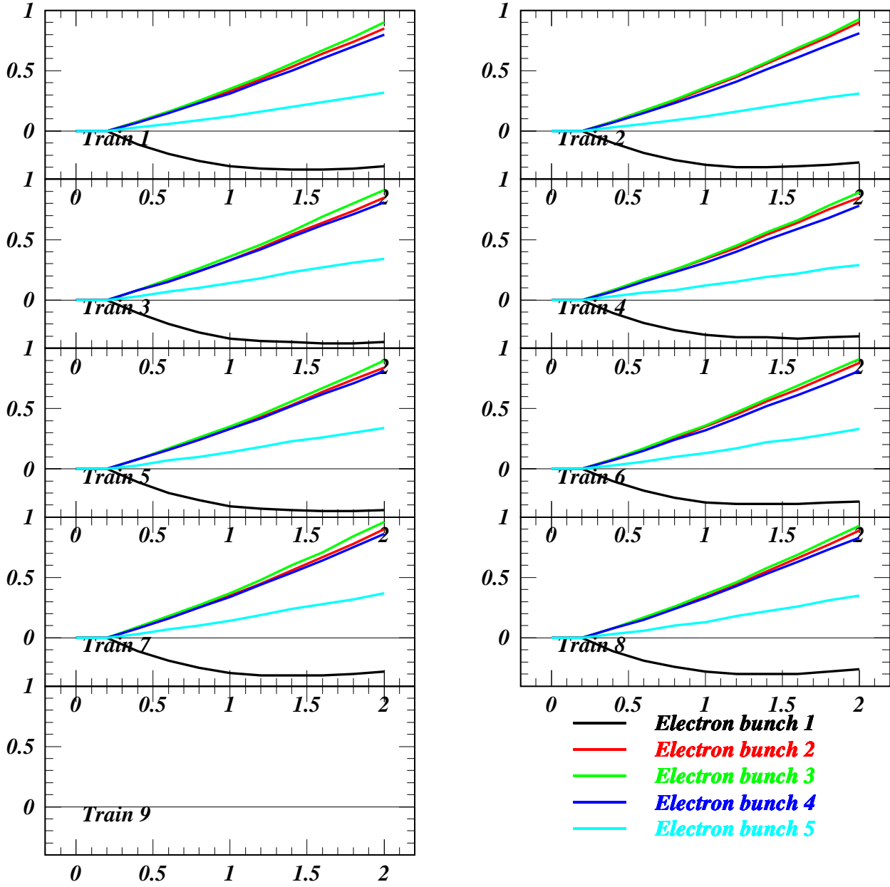
Vertical orbit position at IP ( \mu\text{m} ) vs e^+ Current (mA/bunch) for Job 1623
