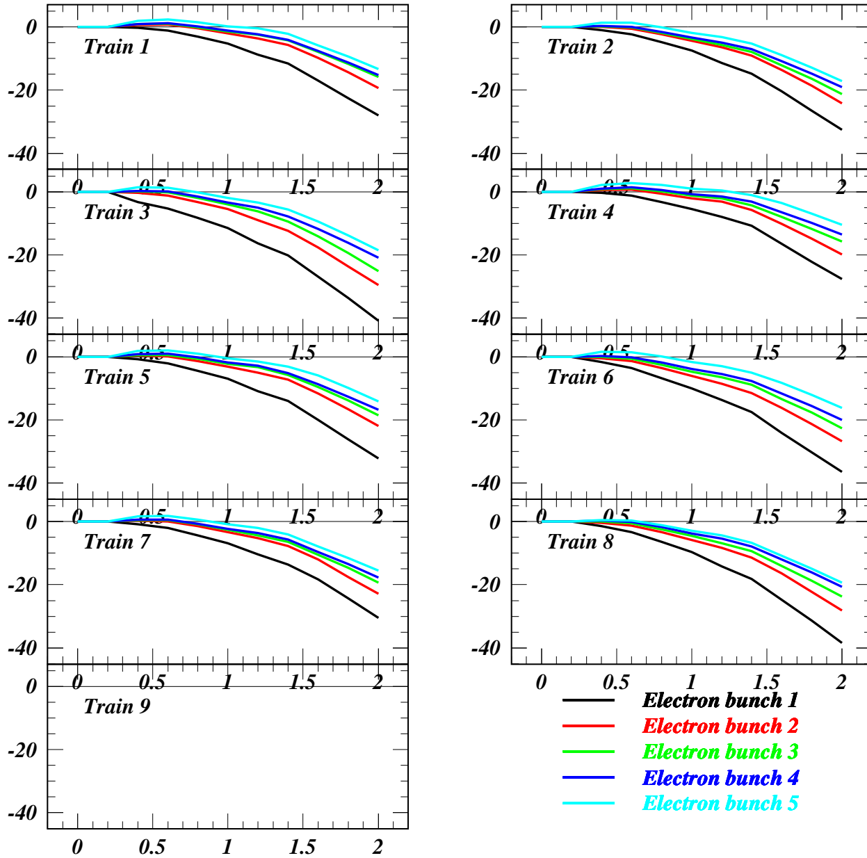
Horizontal orbit position at IP ( \mu\text{m} ) vs e^+ Current (mA/bunch) for Job 1623
