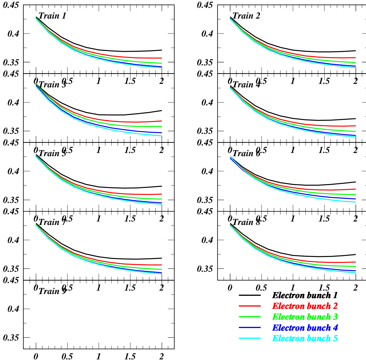
Horizontal Beam Size from \beta at IP (mm) vs e^+ Current (mA/bunch) for Job 1623
