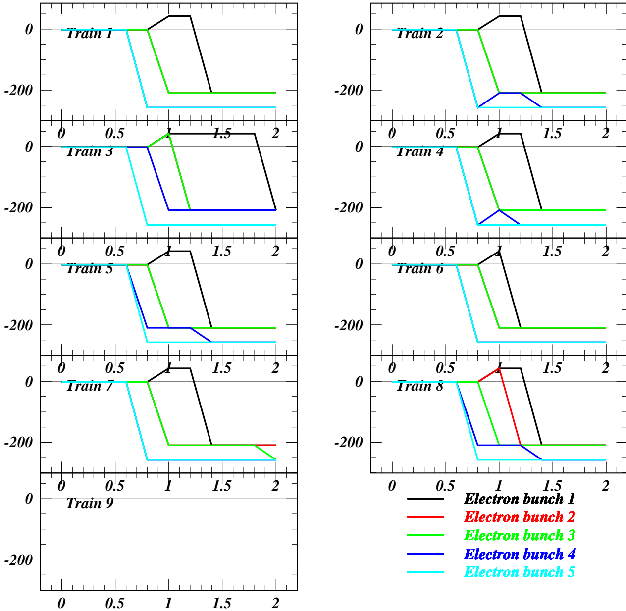
Horizontal \beta_{max} s position vs e^+ Current (mA/bunch) for Job 1623
