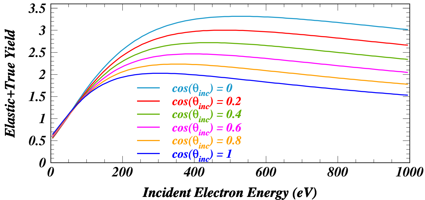
POSINST Elastic+True Yield 50% and Energy Slope of 60.86 eV
