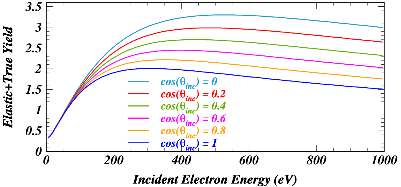
ECLLOUD Elastic+True Yield 50% and Potential Well Energy of 150 eV
