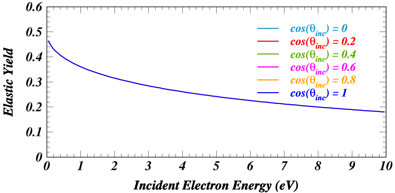
ECLLOUD Elastic Yield 50% and Potential Well Energy of 150 eV
