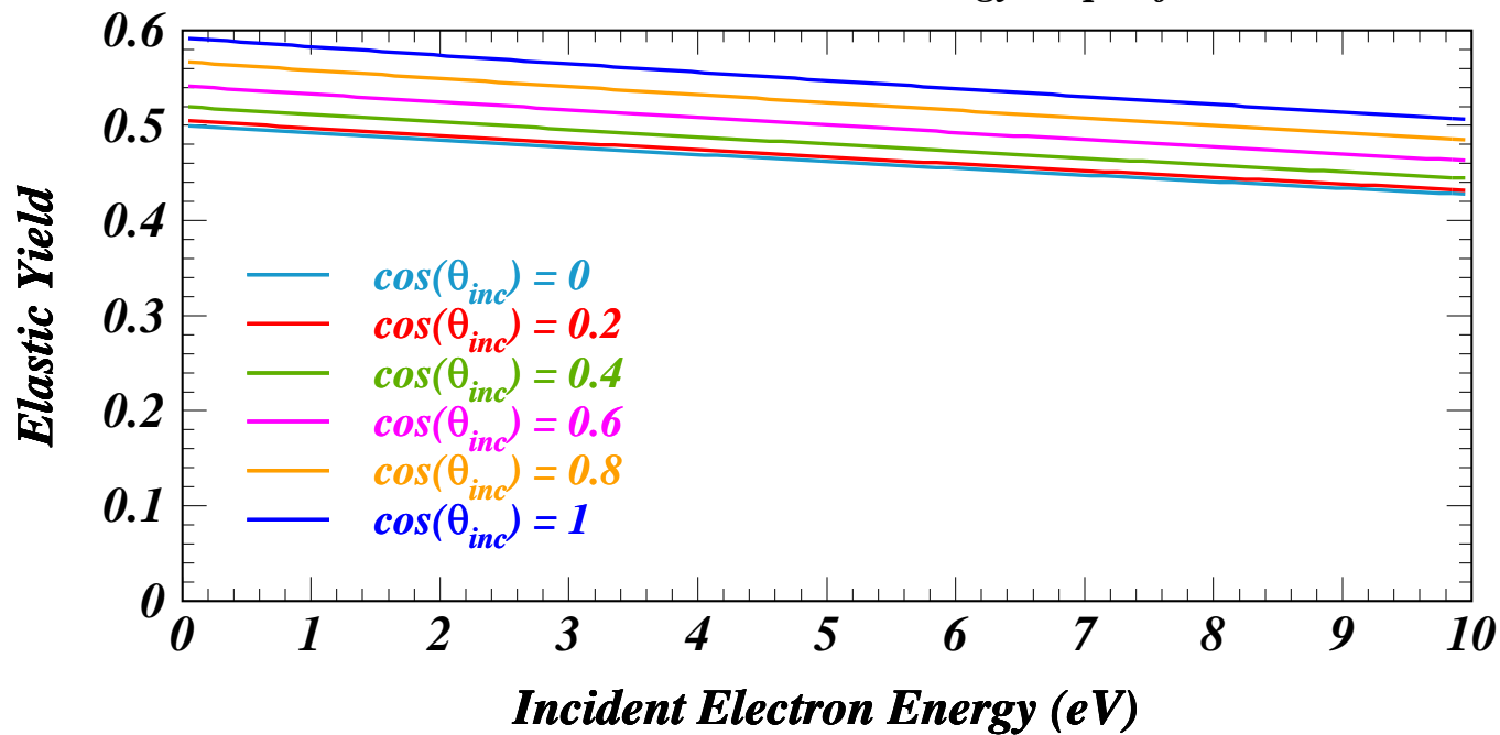
POSINST Elastic Yield 50% and Energy Slope of 60.86 eV
