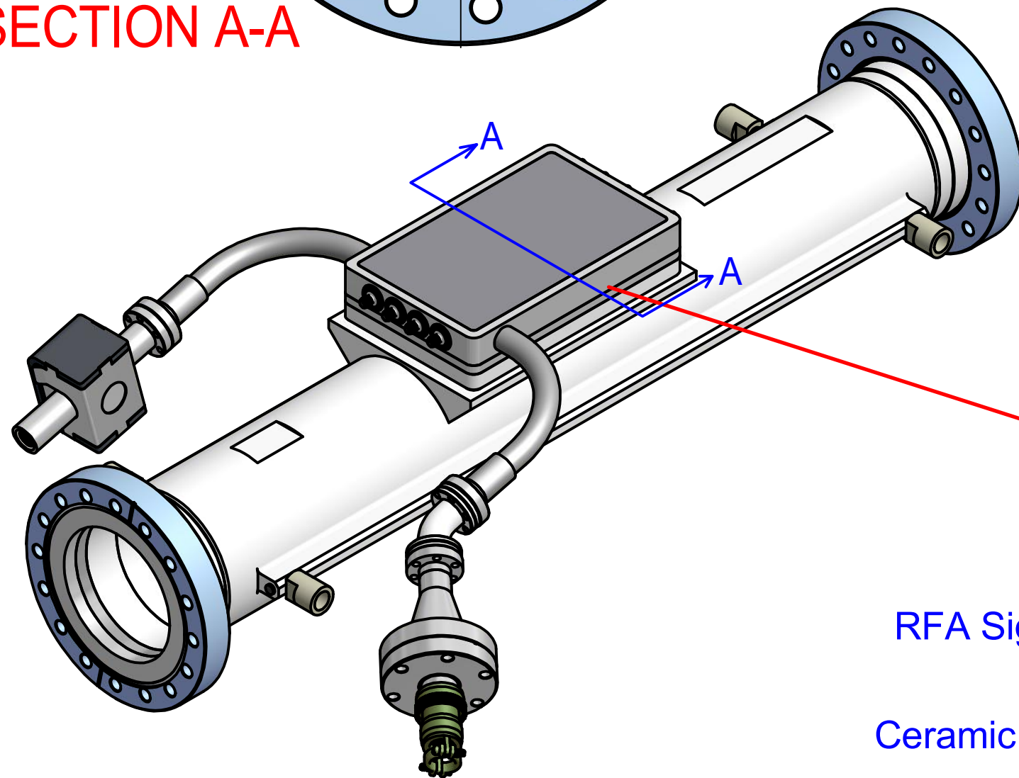
TR-RFA Vacuum Chamber
