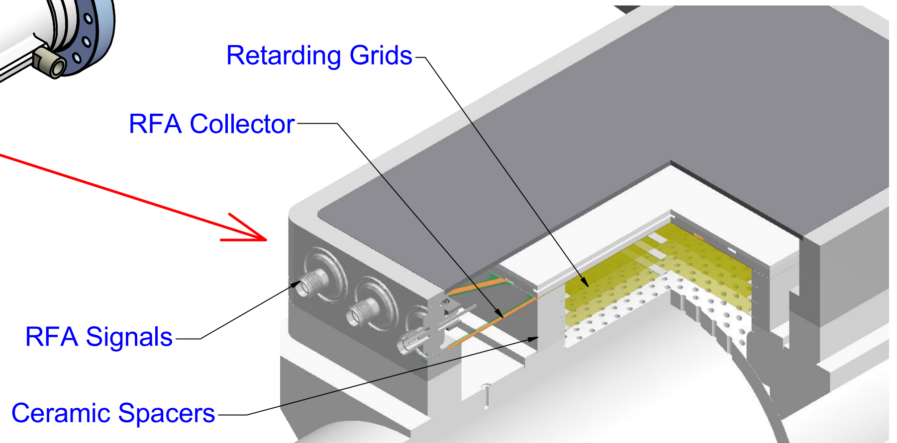
RFA Structure Detail
