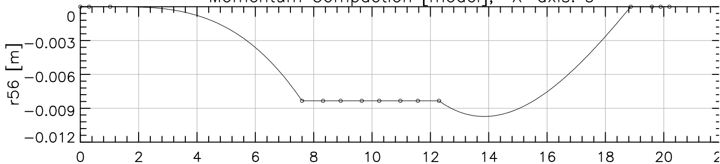
Momentum Compaction [model], X-axis: s
