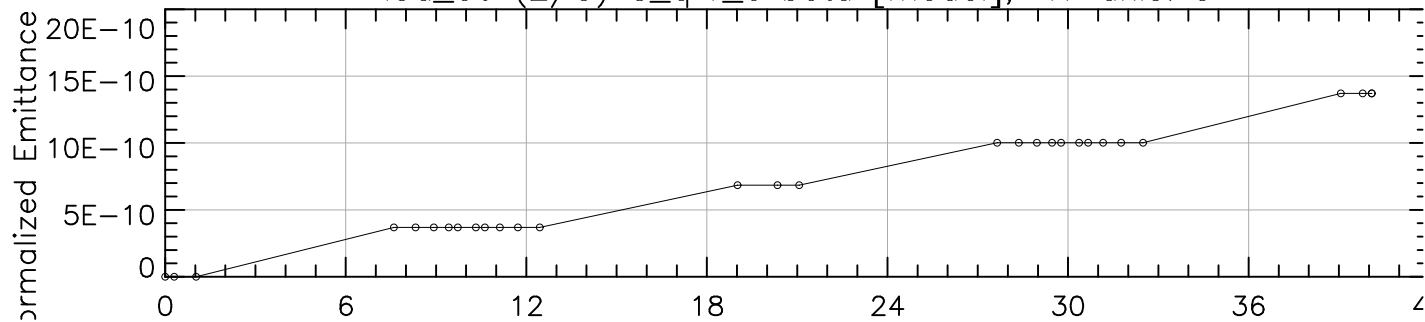
i5a\_e6*(2/3)*C\_q*r\_e*beta [model], X-axis: s
