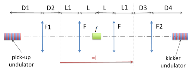
Figure 4: Optical system used to collect and transport the pick-up undulator radiation up to the kicker undulator. The double-arranged lines represent optical lenses ( F_n are the associated focal lengths).
