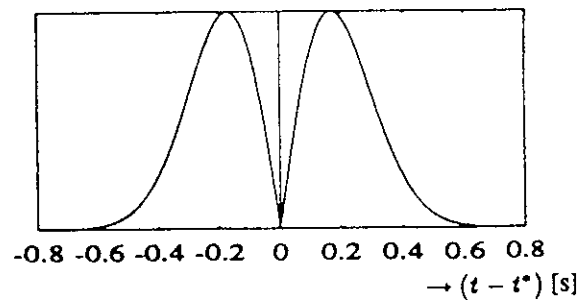
Figure 1: The analytical estimate for the echo shape for a Gaussian energy distribution: \Delta t = 45 ms, \sigma_p = 6 \cdot 10^{-4} and parameters of Table 1.
