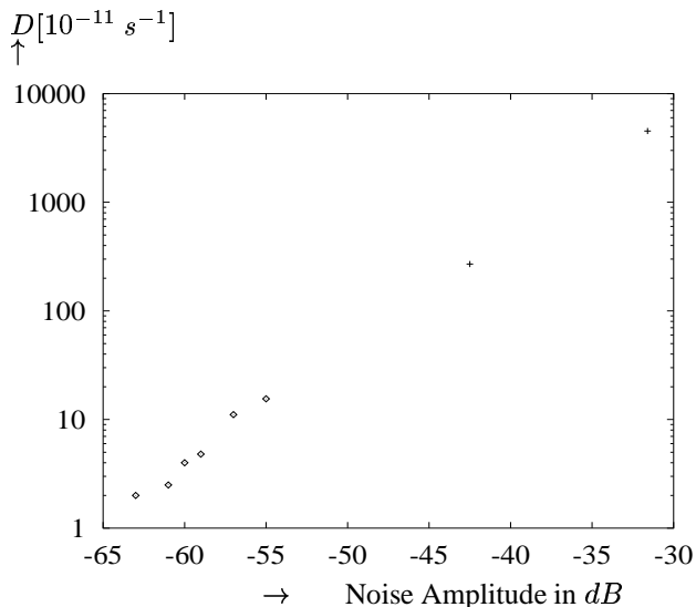
Figure 4: Inferred diffusion coefficients. The vertical axis shows the diffusion coefficients on a logarithmic scale in units of 10^{-11} \text{ s}^{-1} and the horizontal axis the noise amplitude in dB. Assuming a diffusion process with white noise, one expects a straight line with slope 0.1 in this representation. The points with a noise amplitude larger than -45 \text{ dB} are calculated from measurements using the Schottky signal. All other points are calculated from echo measurements.
