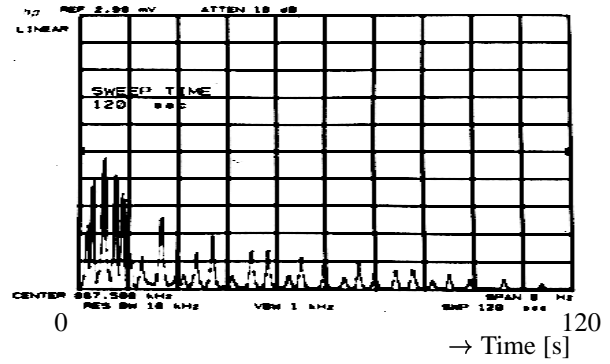
Figure 3: The picture shows the superposition of 22 beam echos for different separation times \Delta t as a function of time after the second RF kick. The time separation of the two RF kicks varies between 5 ms and 220 ms, resulting in an echo response up to two minutes after the second RF-kick.
