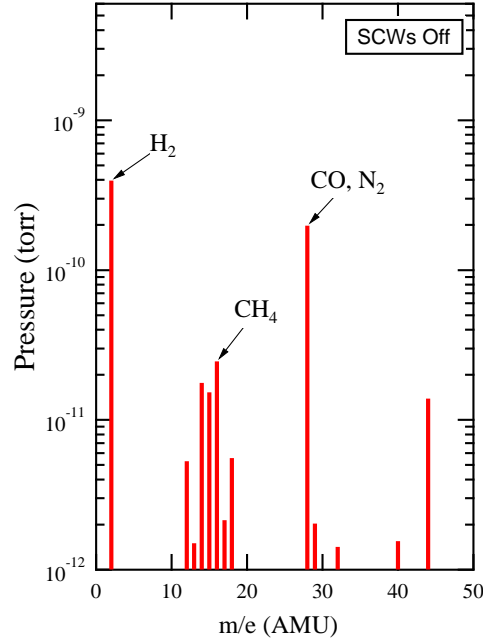
Figure 1.1: A typical gas composition measurement in the Cornell ERL photoinjector.
