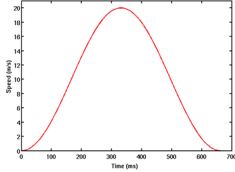
Figure 4.4: The stepper motor was programmed to follow a smooth velocity profile during a scan to avoid any abrupt accelerations which may break the carbon wire [47].
