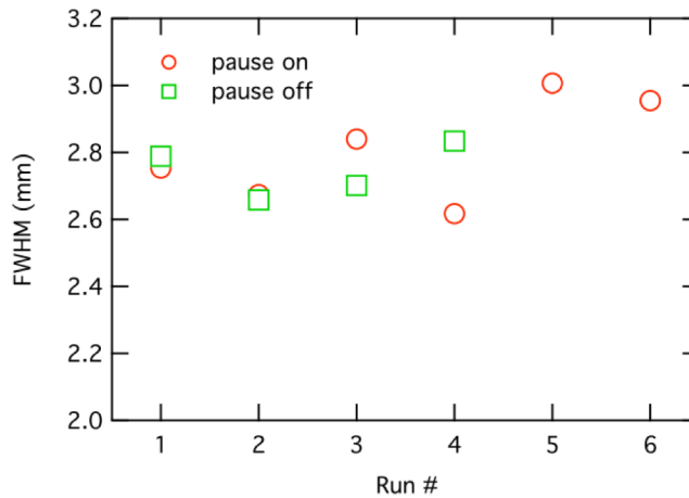
Figure 4.11: A comparison of the full width at half maximum of many beam profiles obtained with and without waiting times between measurements. Circles: Data obtained with a pause of 180 s between consecutive scans – a sufficient amount of time to let wire vibrations decrease to negligible amplitudes. Squares: Data taken with only a 20 s pause, so that the wire did not have time to stop vibrating between scans. Error bars are smaller than the symbol size for all data points [47].
