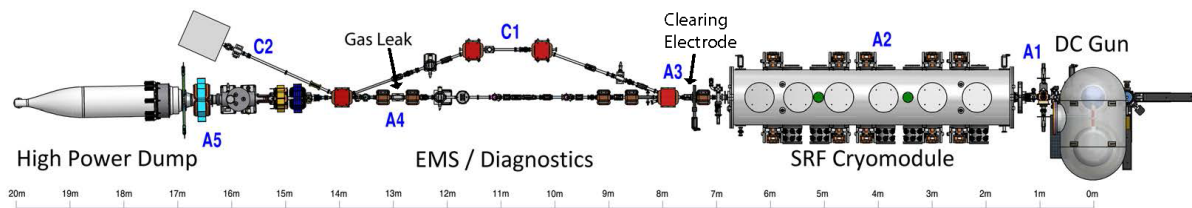
Figure 3.2: A schematic of the photoinjector. The ion clearing electrode was installed just after the beam exists the SRF cavity at A3, and gas was leaked in at the end of A4. Radiation measurements were taken at several locations between sections A3 and A4 (next to the beam pipe). (Note that this figure was previously used in section 1.3 Fig. 1.3 to illustrate a separate point).
