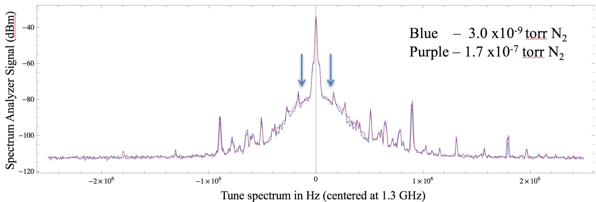
Figure 2.2: A beam spectrum taken while N_2 gas was leaked into the vacuum chamber of the Cornell ERL photoinjector at two different pressures. Equation (1.12) predicts that, for a 10 mA, 2 mm beam, beam-ion coupling should produce peaks in the 10-100 kHz range. For N_2 , the location of the expected peaks is indicated with blue arrows. However, these peaks are unobservable due to large amounts of background noise induced by the photoinjector's RF systems at the time of the experiment. Increasing the vacuum pressure from 3.0 \times 10^{-9} torr to 1.7 \times 10^{-7} torr had very little effect on these observations.
