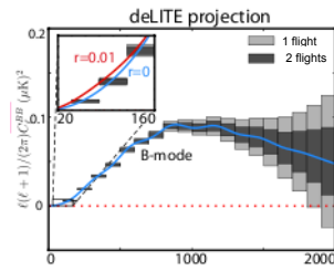
Fig. 5. Projected deLITE errors from realistic simulations.
